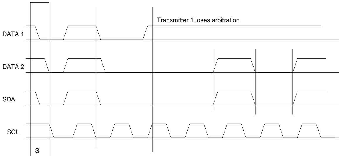
Figure 5.2: SMBus arbitration
